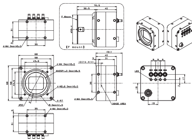
STC-CMB/CMC120ACXP STC-CMB120ACXP-F/CMC120ACXP-F
