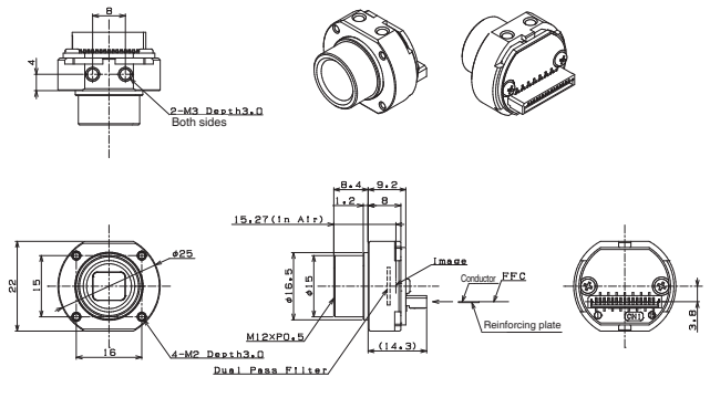
STC-S133MIP-L(DL)
